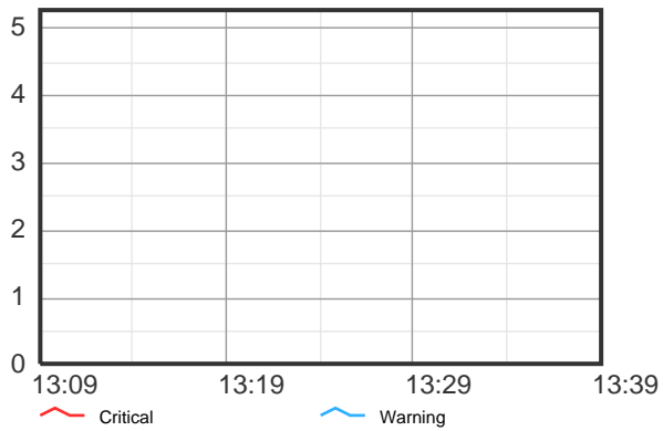
Log Warnings
