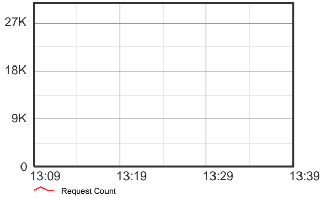
Request Count
