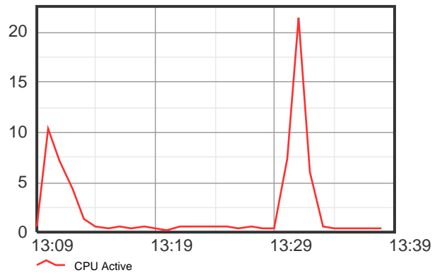
CPU
