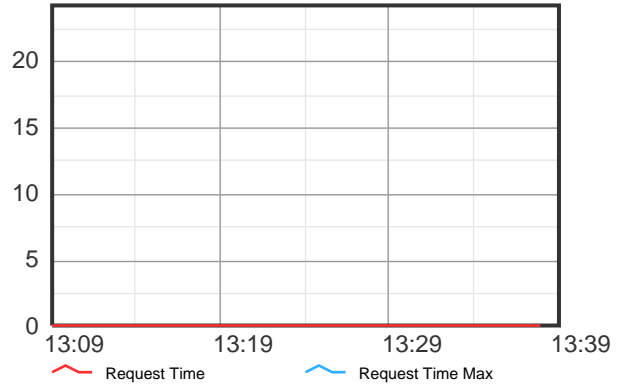
Request Time
