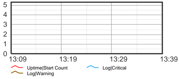
Server 00 - app-0
